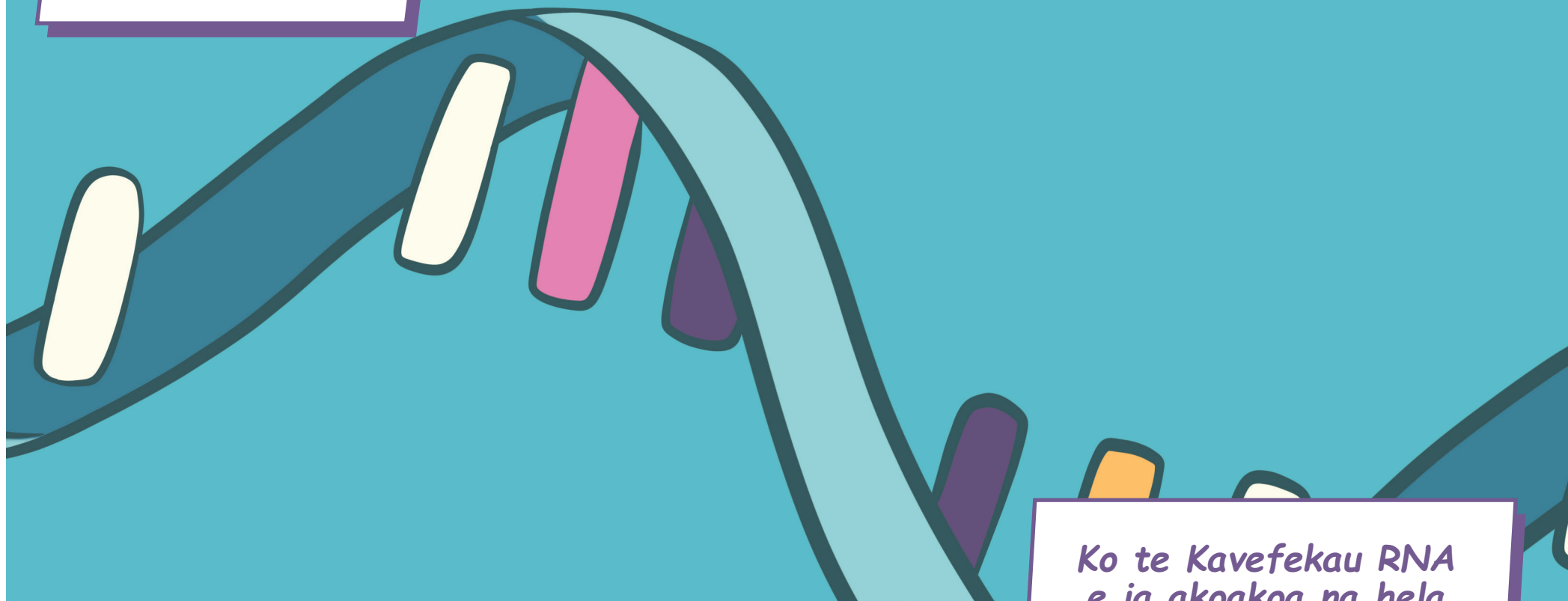
Kavefekau RNA
